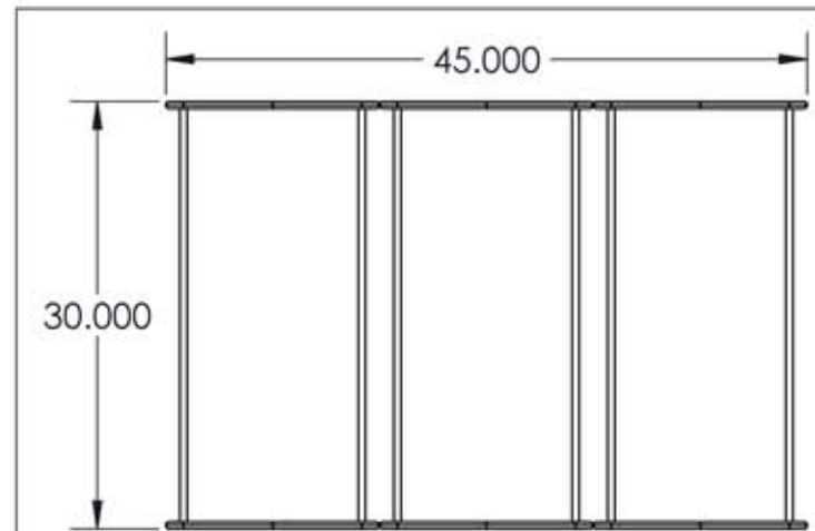
FRONT VIEW OF THREE CAN LINERS
